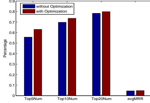
Figure 5.9: ACM data set: Parameter Optimization
