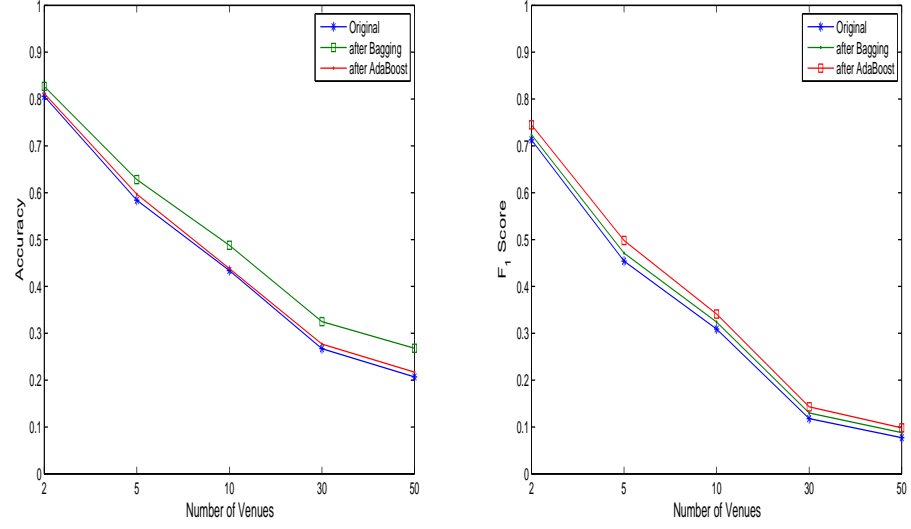
Figure 5.5: Bagging and Boosting: Accuracy and F_1 Score for ACM data
