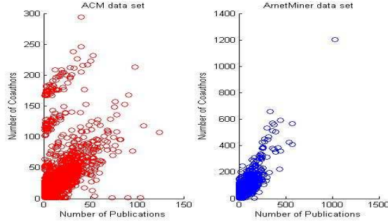
Figure 7.1: Correlation between Number of Publications and Coauthors
