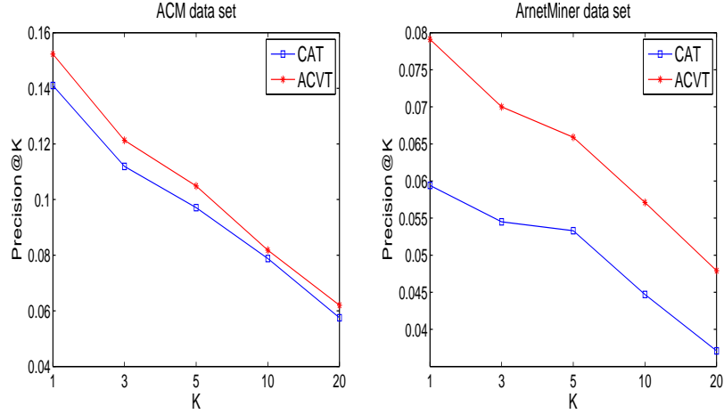
Figure 6.6: Cited Autor Prediction: Precision@K
