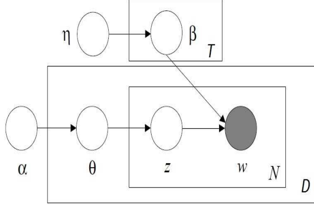
Figure 4.1: Graphical Model for LtoRTM
