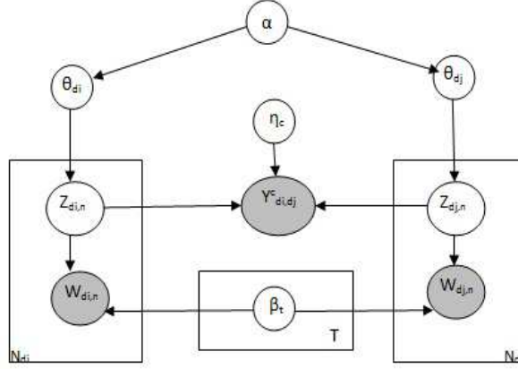
Figure 4.2: Graphical Model for LtoRTM
