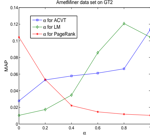
Figure 6.5: Combine ranking methods (ArnetMiner data set)
