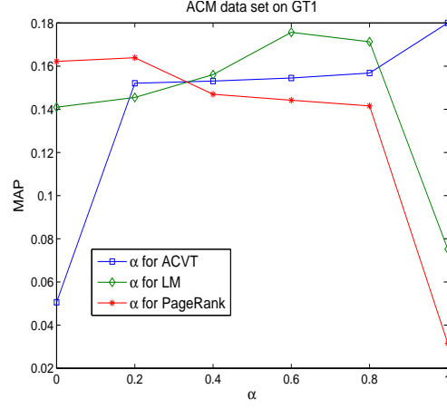
Figure 6.4: Combine ranking methods (ACM data set)
