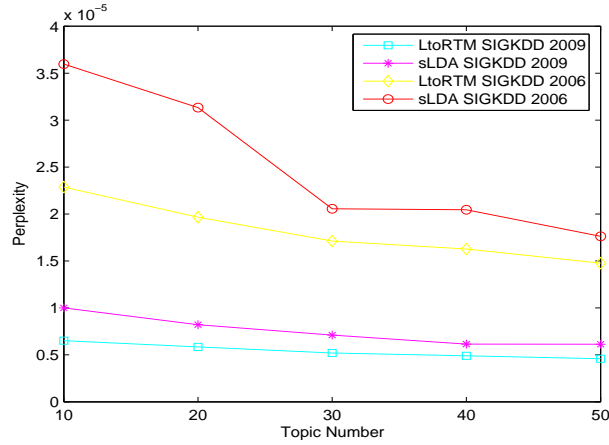
Figure 4.6: Perplexity
