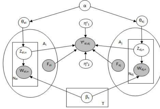
Figure 4.3: Graphical Model for LtoRTMF
