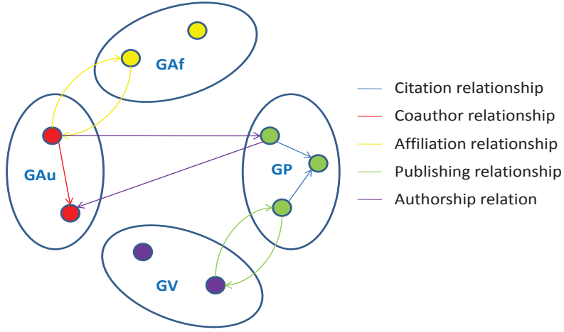
Figure 3.2: Multi-type (4-TV2) Citation Network
