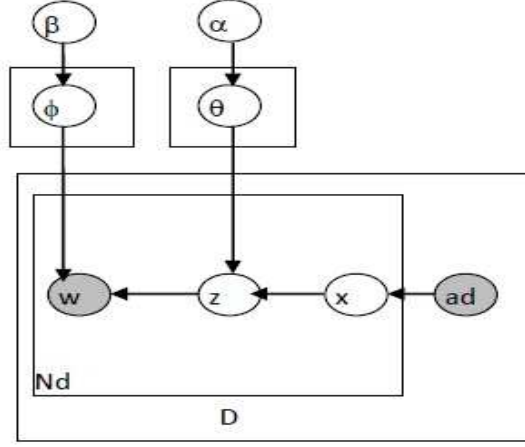
Figure 6.1: Graphical Model for the original Author-Topic Model
