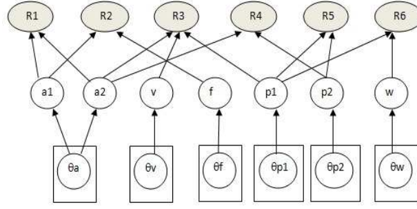
Figure 7.5: Graphic Model Representation
