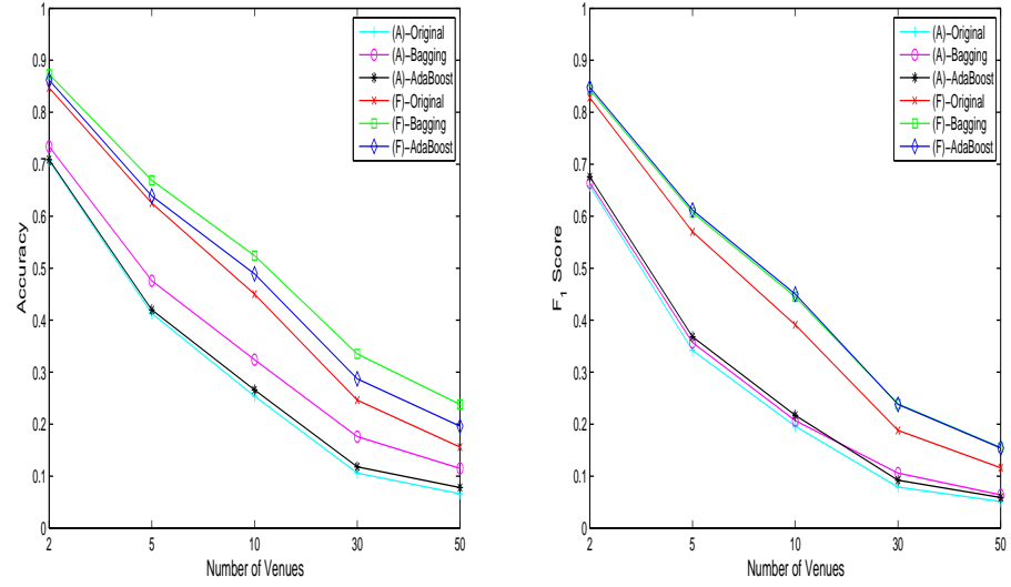
Figure 5.6: Bagging and Boosting: Accuracy and F_1 Score for CiteSeer data
