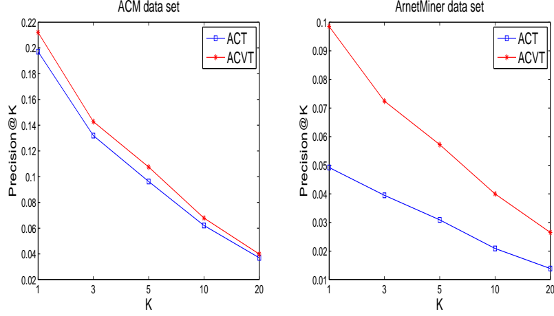
Figure 6.7: Venue Prediction: Precision@K
