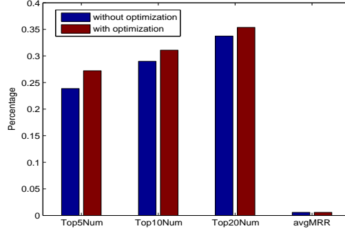
Figure 5.10: CiteSeer data set: parameters optimization
