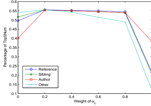
Figure 5.7: ACM data set: Weight of Neighbors
