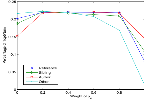
Figure 5.8: CiteSeer data set: Weight of Neighbors
