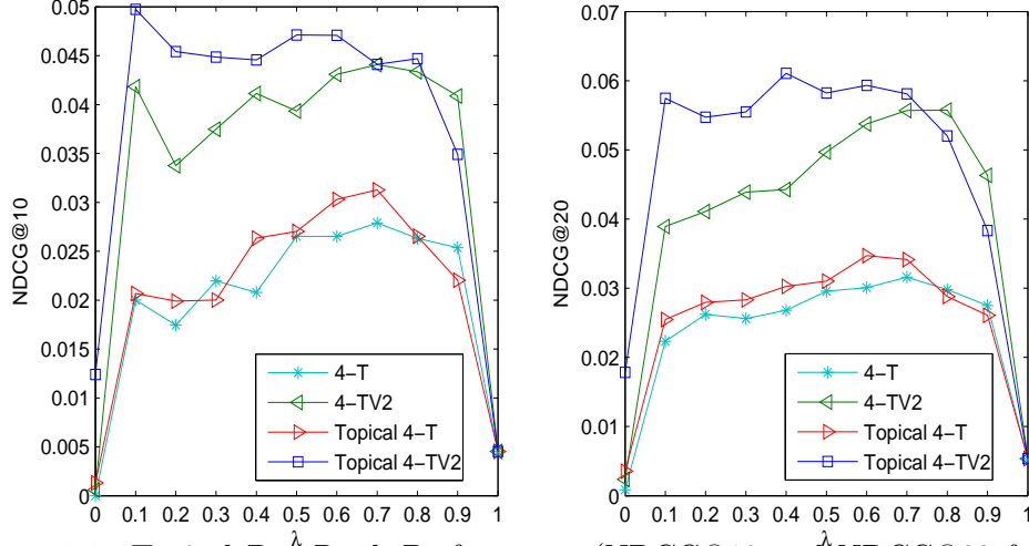
Figure 3.9: Topical PageRank Performance (NDCG@10 and NDCG@20 for PC members) as the BM25 weight ( \lambda ) is varied.
